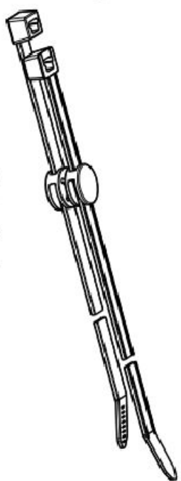
Isometric view Scale: 1:2
