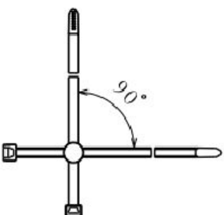
Free bundle orientation Cable tie position admitted into 90° area
