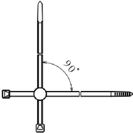
Free bundle orientation Cable tie position admitted into 90° area
