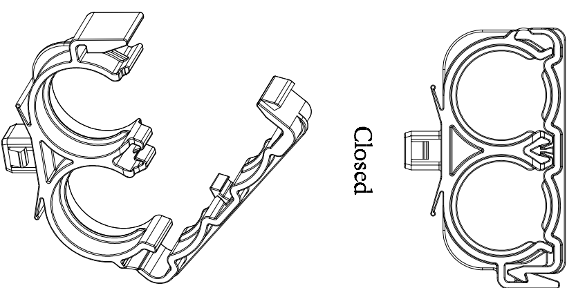
Isometric view
